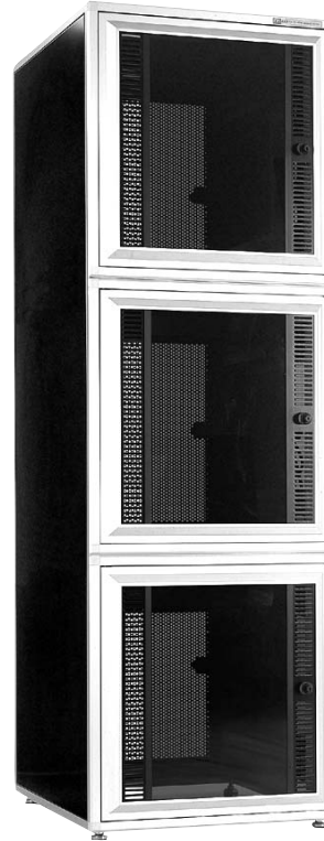
Patented, reversible 3-channel raceway on each side of cabinet separates power and data cables for each compartment
